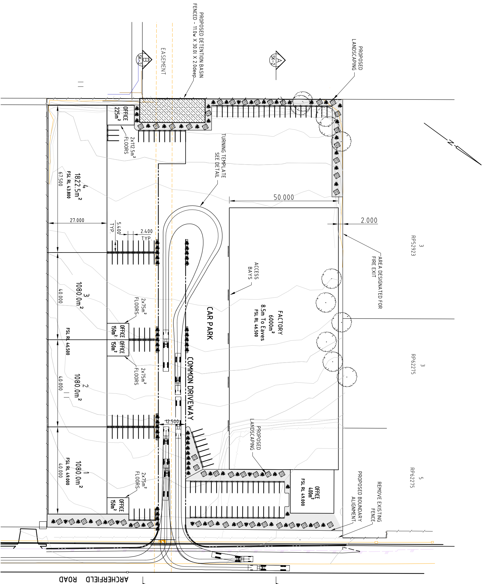
LAYOUT PLAN 1:500
